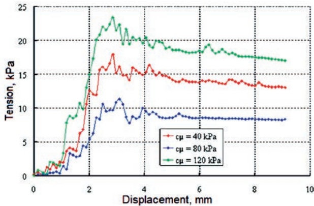
FIGURE 6. Pressure-displacement curves for different values of micro-cohesion.
